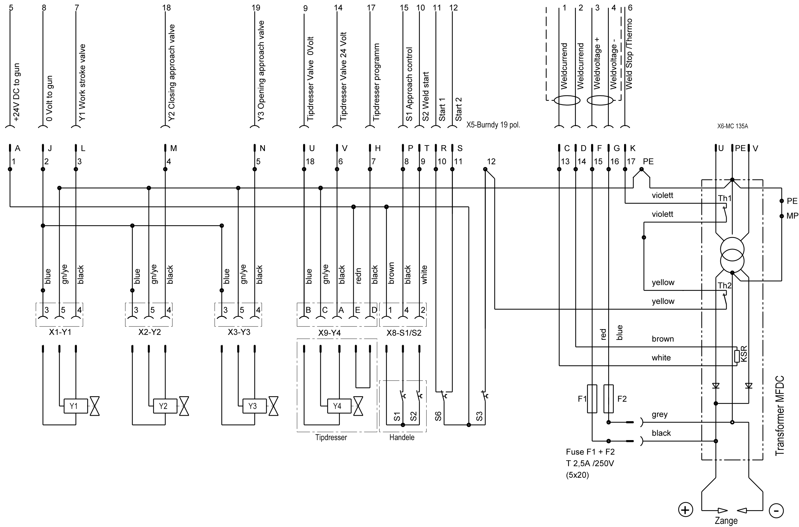
Circuit diagram
